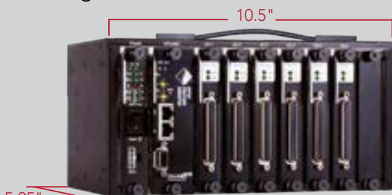
DNR-ECAT-600 (HALF RACKtangle) 160,000 hours
