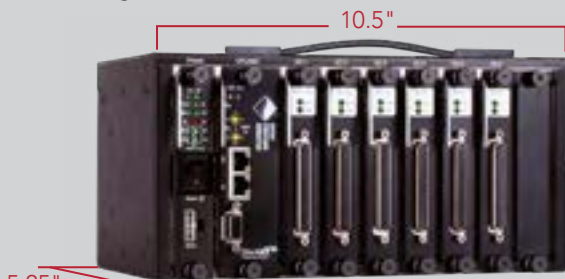
DNR-ECAT-600 (HALF RACKtangle) 160,000 hours
